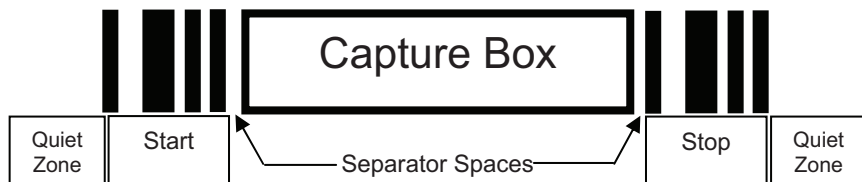
Figure 27 CapCode Structure
